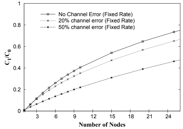
Fig. 8. The impact of channel errors on C_1/C_0 with respect to the number of contending stations (homogeneous environment)
