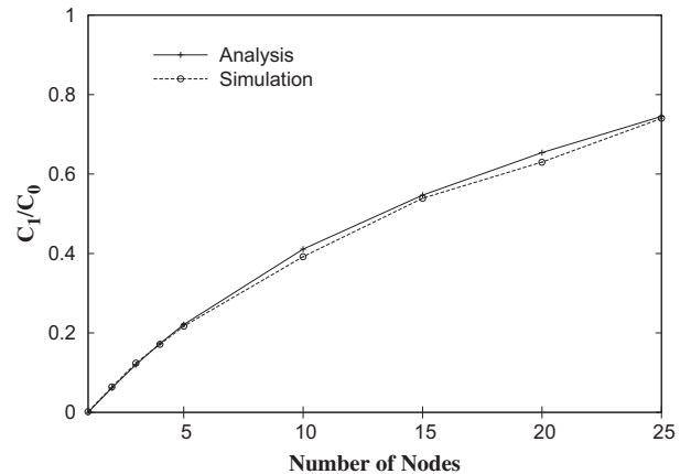
Fig. 10. C_1/C_0 as a function of N : Analysis vs. Simulation
