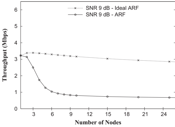
Fig. 3. Performance of ideal ARF ( \theta_u=10, \theta_d=2 ) at SINR=9dB (1000 bytes)
