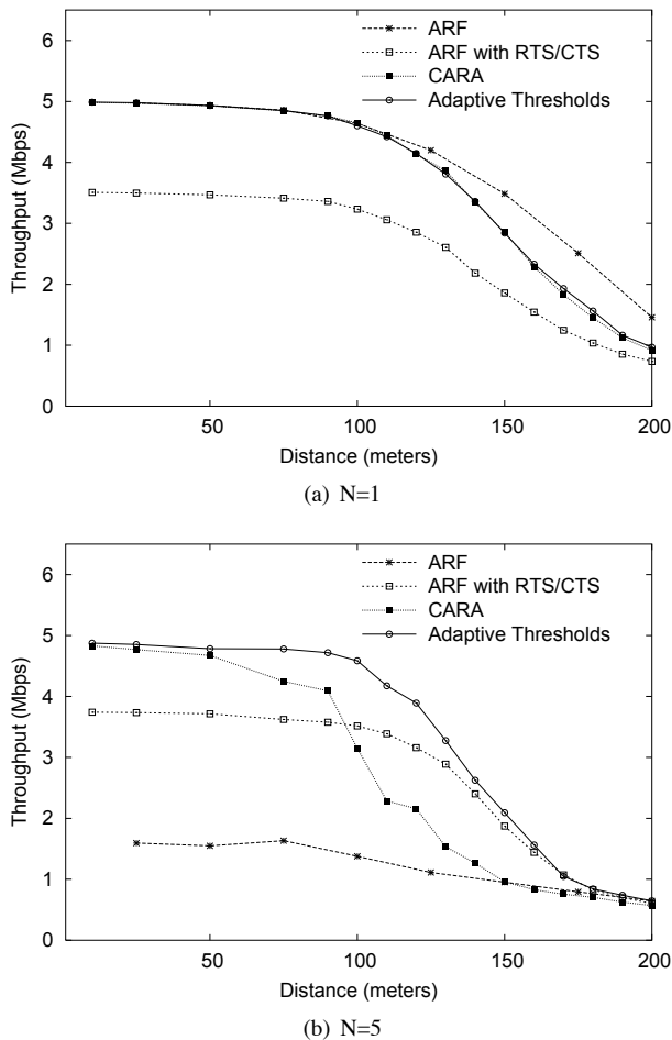
Fig. 12. Throughput comparison in Ricean fading channel (payload = 1000 bytes) for N=1 and 5
