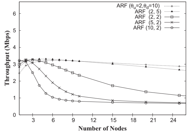
Fig. 2. ARF-DCF throughput for various \theta_u and \theta_d combinations at SINR=9dB (1000 bytes)
