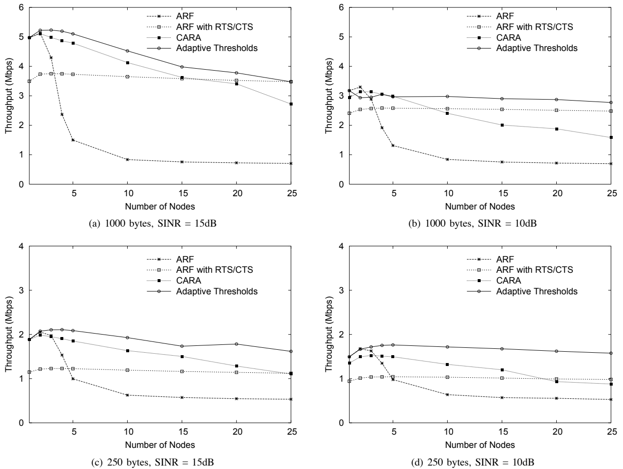
Fig. 11. Throughput comparison of our proposal (Adaptive Thresholds) against ARF, ARF with RTS/CTS, and CARA in stationary channel condition at which (a) SINR=15dB, 1000 bytes (b) SINR=10dB, 1000 bytes (c) SINR=15dB, 250 bytes (d) SINR=10dB, 250 bytes
