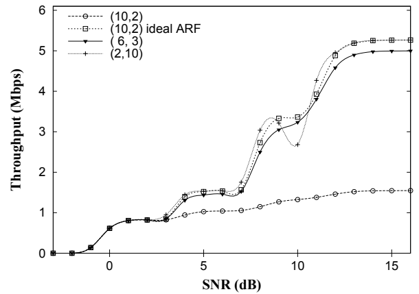
Fig. 5. ARF-DCF throughput for various \theta_u, \theta_d combinations under N = 5
